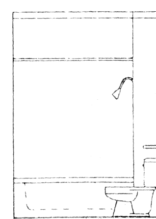
26 NORTH 27 WEST/EAST 28 SOUTH 29 EAST/WEST BATH 1 END UNIT (BLDG 5) @ 1/4" = 1'-0"
