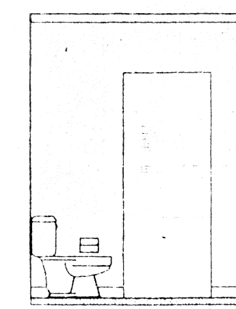
6 NORTH 7 WEST/EAST 8 SOUTH MASTER BATH TYP. UNIT (BLDGS 1-4) @ 1/4" = 1'-0"
