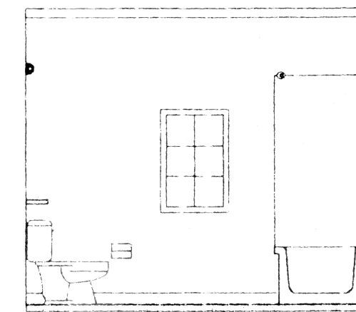
10 NORTH 11 WEST/EAST BATH 1 END UNIT (BLDGS 1-4) @ 1/4" = 1'-0"
