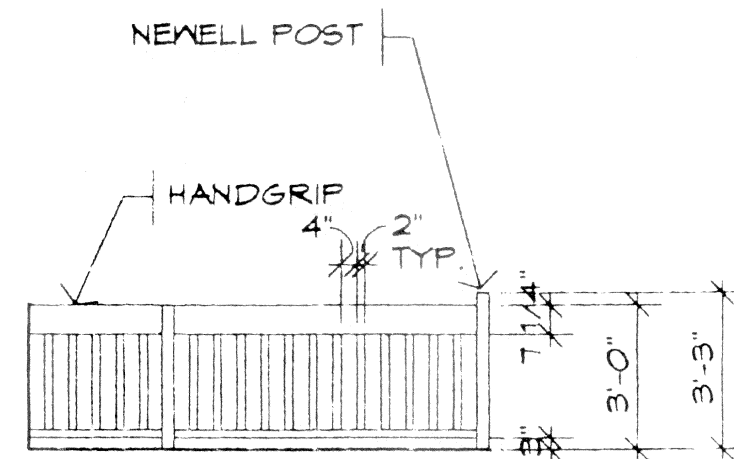
1 UPPER LEVEL END UNIT HANDRAIL BLDGS 1-4 @ 1/4" = 1'-0"
