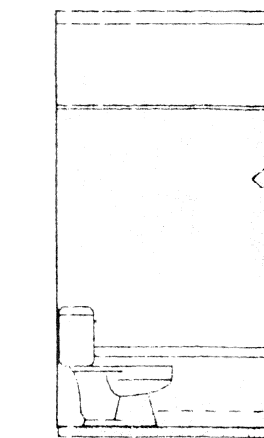
14 NORTH 15 WEST/EAST 16 SOUTH MASTER BATH TYP. UNIT (BLDGS 1-4) @ 1/4" = 1'-0"
