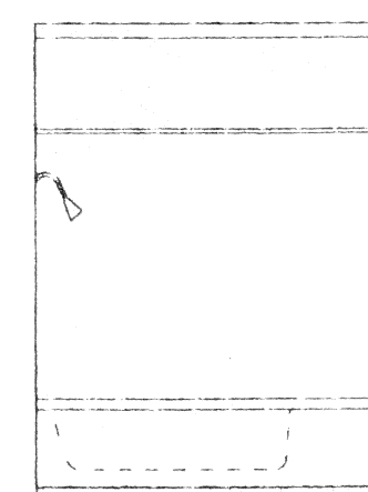
18 NORTH 19 WEST/EAST MASTER BATH TYP. UNIT (BLDG 5) @ 1/4" = 1'-0"
