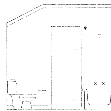
18 NORTH 19 WEST/EAST MASTER BATH TYP. UNIT (BLDG 5) @ 1/4" = 1'-0"
