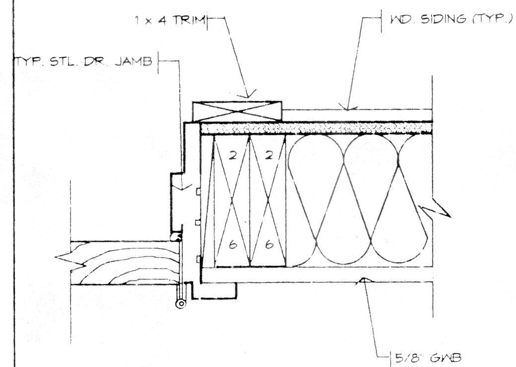
19 EXT. DOOR JAMB @ 3" = 1'-0" 93184
