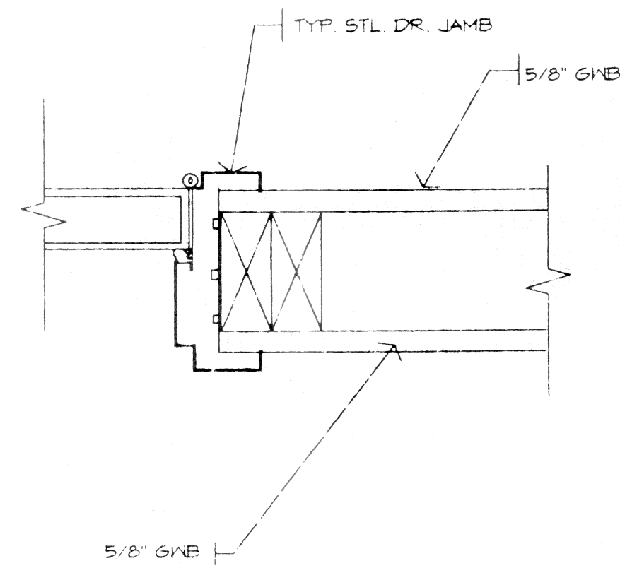
20 INT. DOOR JAMB @ 3" = 1'-0" 93184
