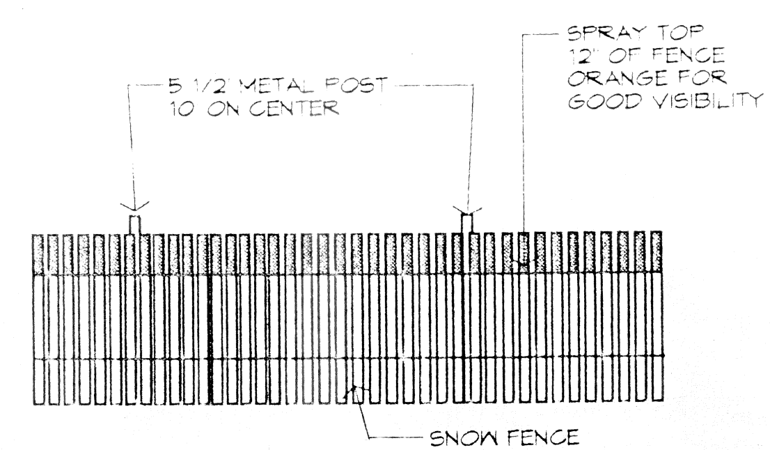
35 CONSTRUCTION FENCE @ 1/4" = 1'-0" 93184
