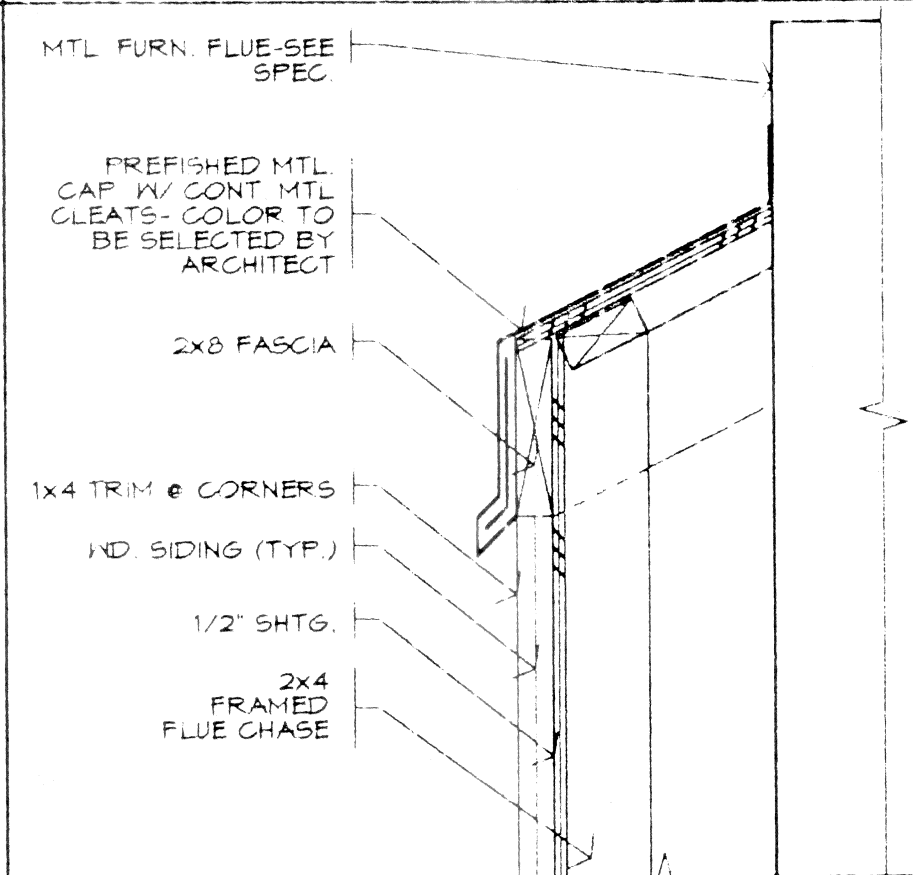
30 FURNACE FLUE CHASE @ 1 1/2" = 1'-0" 93184
