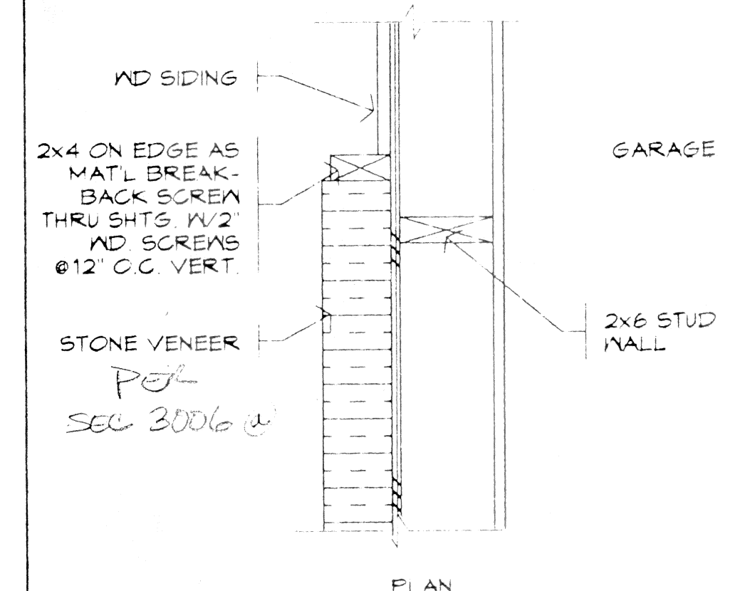
29 STONE RETURN @ ENTRY @ 1 1/2" = 1'-0" 93184
