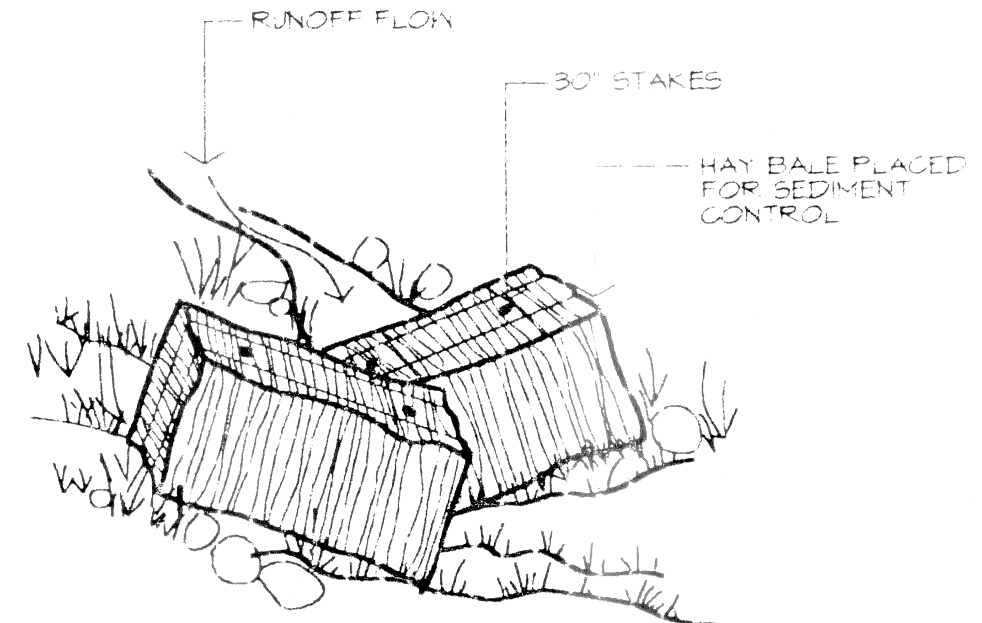
31 EROSION BALE DETAIL @ 1/4" = 1'-0" 93184
