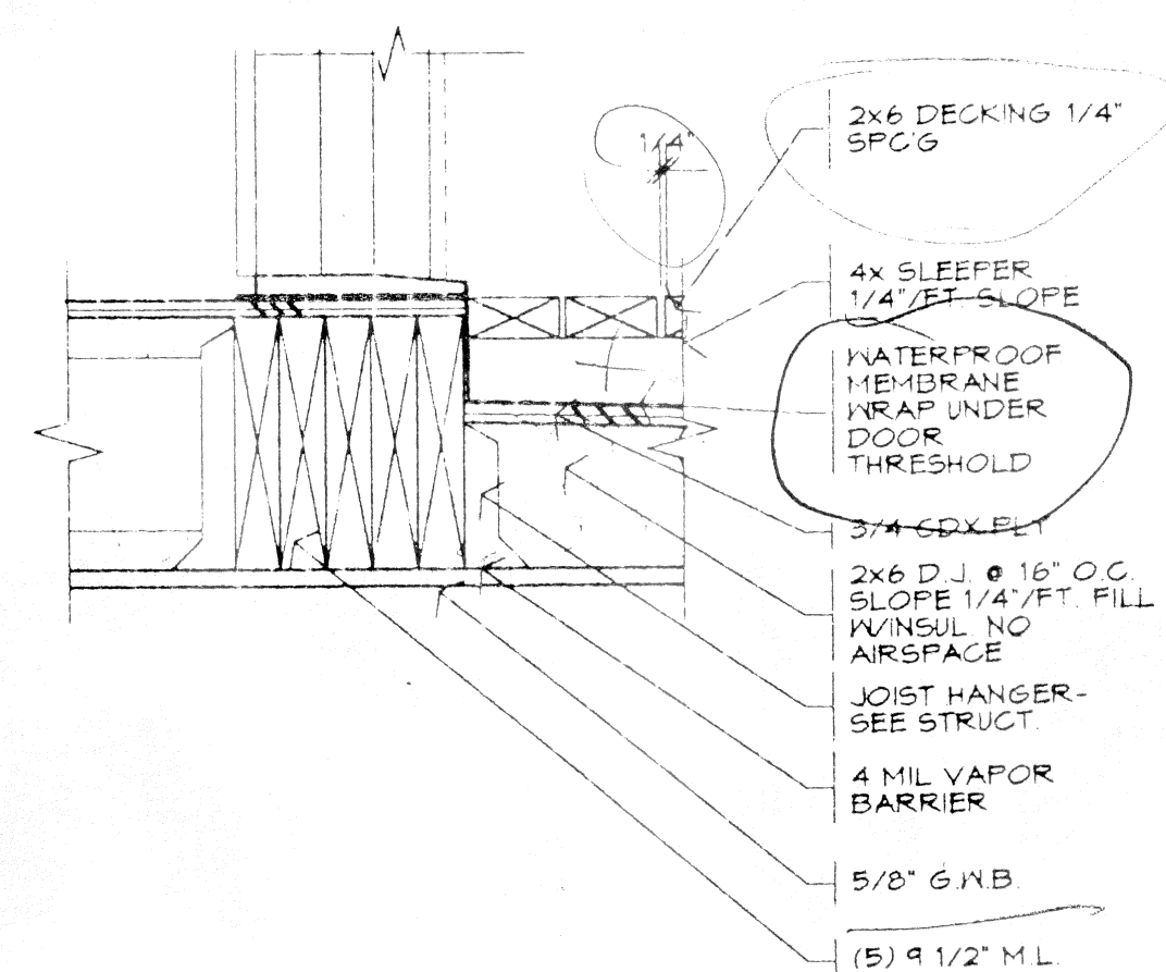
34 DECK SECTION @ 1 1/2" = 1'-0" 94103
