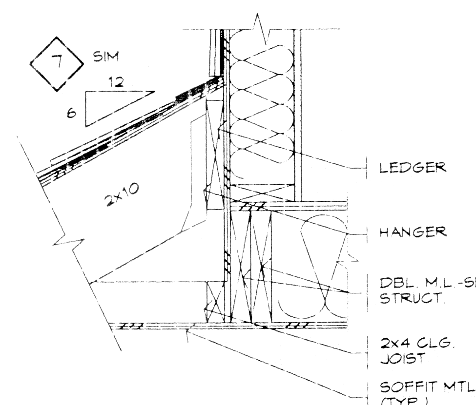
25 ENTRY ROOF @ WALL @ 1 1/2" = 1'-0" 93184
