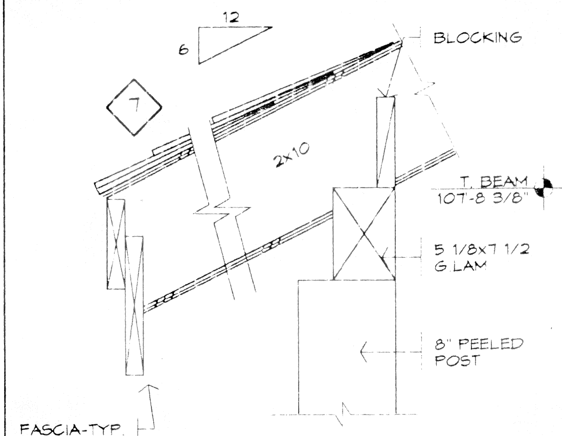
24 ENTRY ROOF DETAIL @ 1 1/2" = 1'-0" 93184
