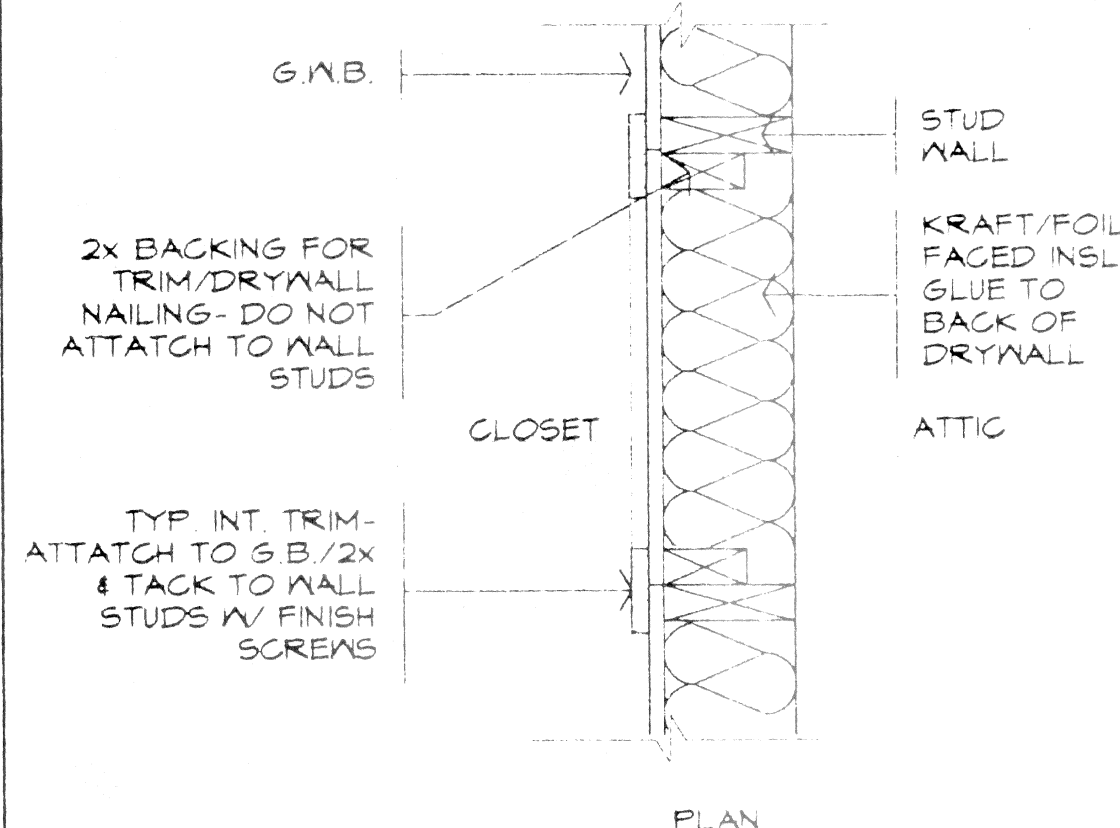
26 ATTIC ACCESS IN WALL/CLG. @ 1 1/2" = 1'-0" 93184
